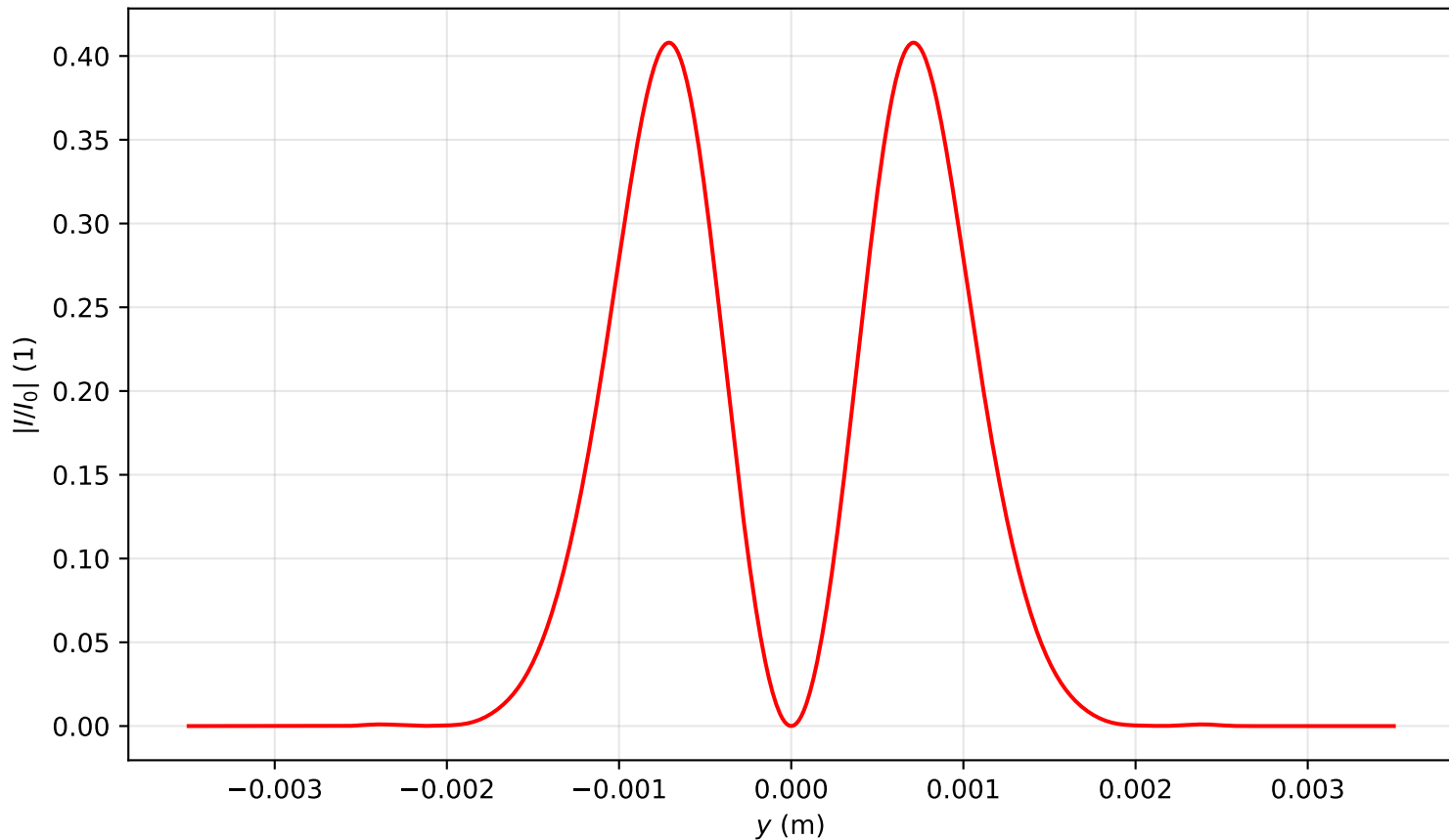
Intensity profile I(x=0, y, z=2.309)/I_0 , P_{in}=2.0P_{cr} , artificial time
